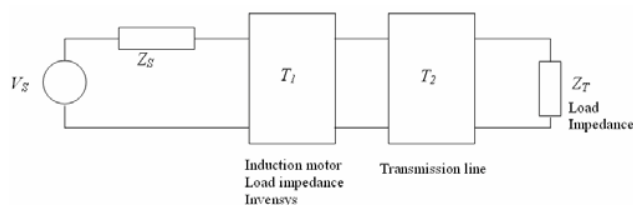
Fig. 2 Two-port Modeled of Power-line As Data Channel
