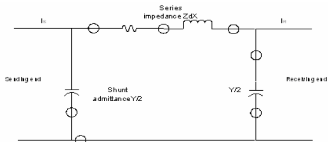
Fig. 1 Equivalent II model for transmission line
