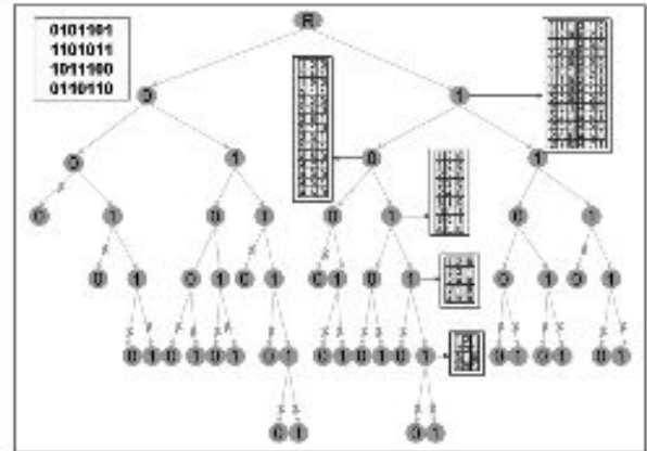
Fig. 2 An example of consensus tree with d = 1, \Sigma = \{0,1\} and S = \{0101101, 1101011, 1011100, 0110110\} . N = 4, L = 7 and |\Sigma| = 2, q = 4, d = 1
