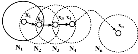
Fig. 2 Mechanism of Tabu list
