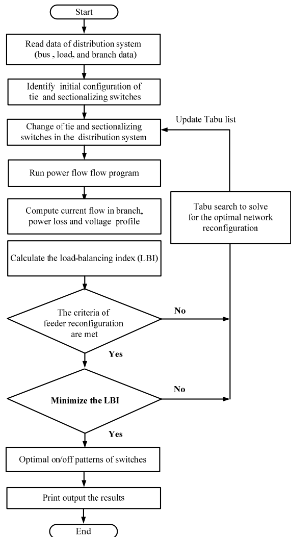
Fig. 4 Flowchart of network reconfiguration for load balancing
