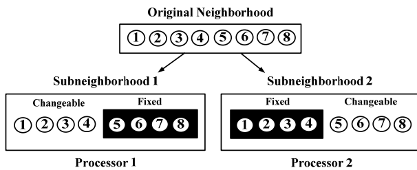
Fig. 3 Search direction of Tabu search
