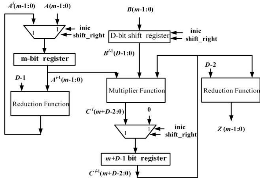
Fig. 4 Block diagram of the LSD multiplier implemented in this work
