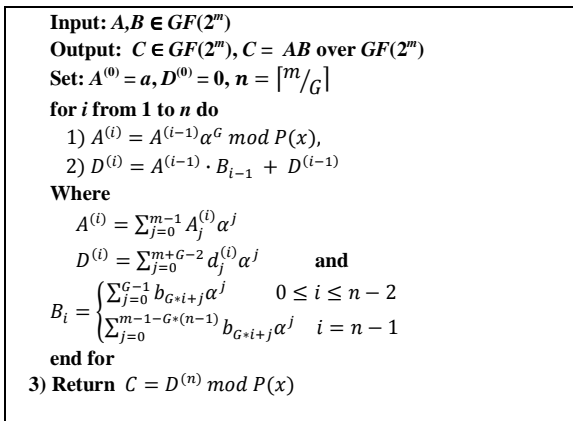
Fig. 3 The LSD multiplication algorithm [7]
