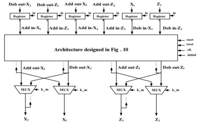
Fig. 7 Architecture of point addition and doubling iteration LD based on the key bits
