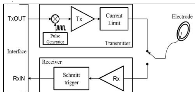
Fig. 3 Block diagram of pulse communication system which consisted of electrode, interface, transmitter and receiver
