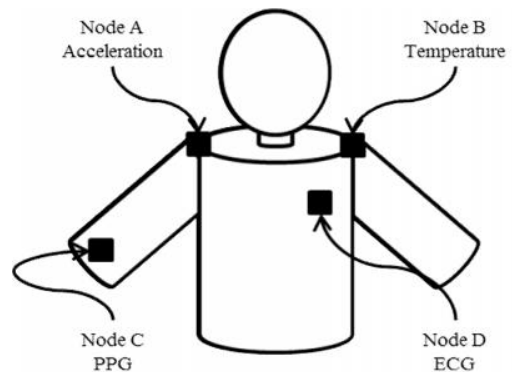
Fig. 2 Each bio-sensing unit functions as a node in communication network and four nodes formed a wireless personal area network
