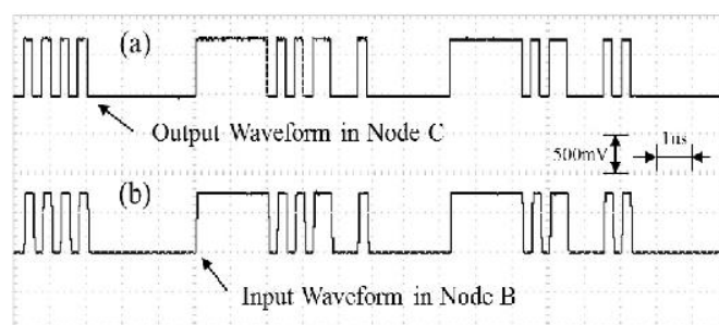
Fig. 4 Pulse waveform between Node B and Node C. It shows a frame including PPG data
