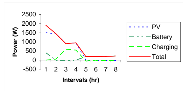
Fig. 5 The primary and secondary energy sources
