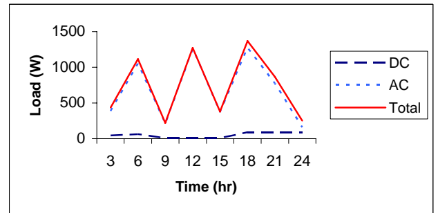
Fig. 4 The various required load
