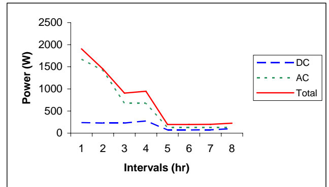
Fig. 3 The various required load
