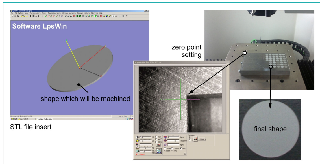
Fig. 2 The engraving tests on Al7075 plate
