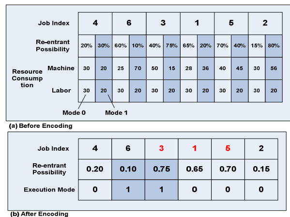
Fig. 1 Multi-level chromosome encoding
