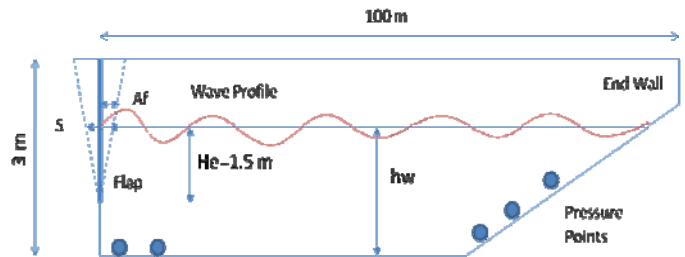
Fig. 3 Flap Type Wave Maker
