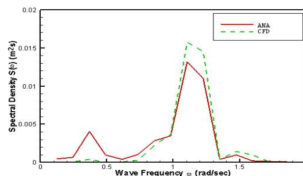
Fig.. 9 Comparison of Wave Spectrum for 1:20:1
