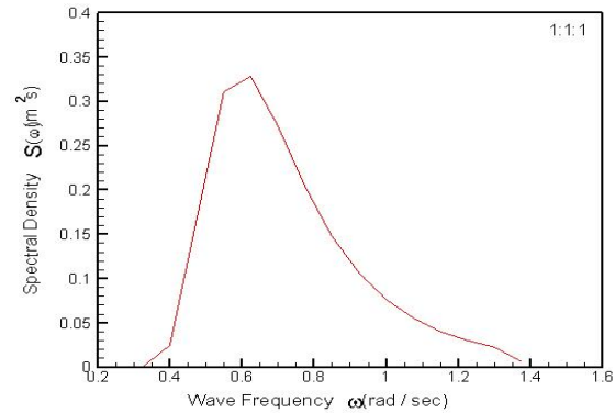
Fig.. 5 The Bretschneider Wave Spectrum [H_s = 1.5 \text{ \& } T_z = 7.5]
