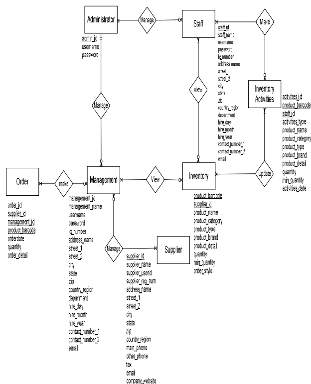
Fig. 3 E-R diagram of MBIMS
