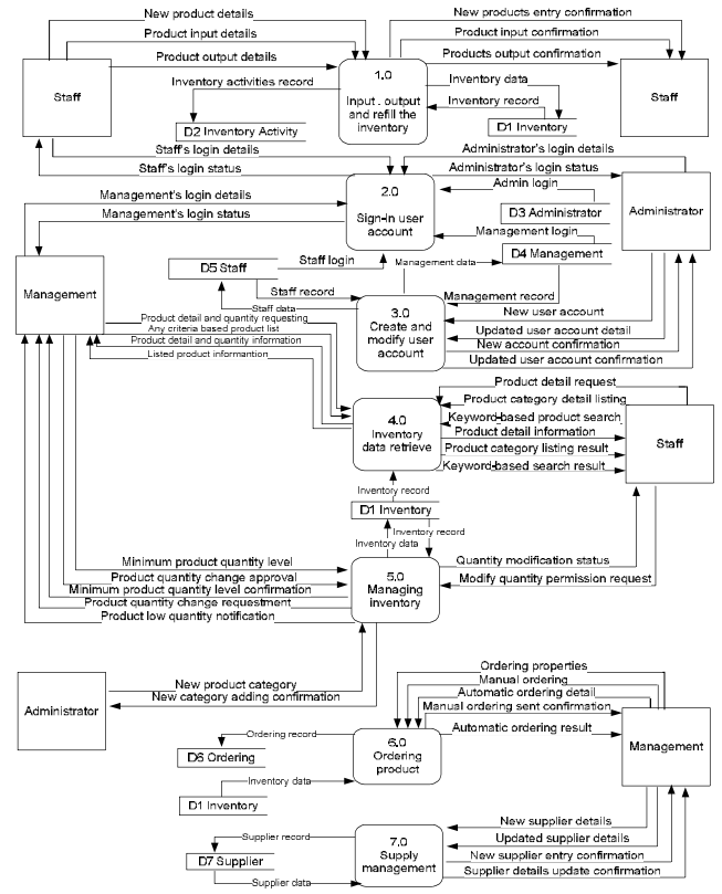
Fig. 2 Level-0 diagram of MBIMS
