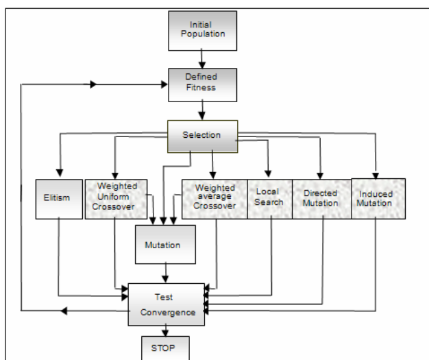
Fig. 1 Algorithm
