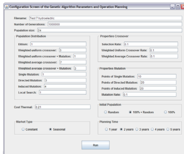
Fig. 11 Screen configuration data used by GAs
