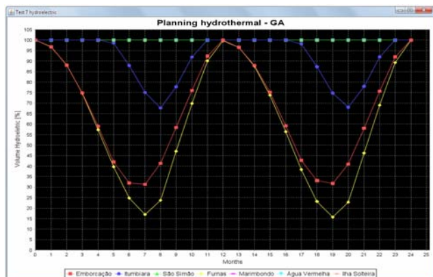
Fig. 12 Planning Hydrothermal
