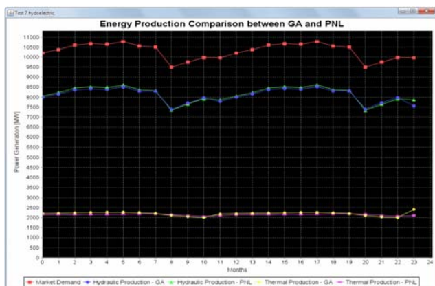
Fig. 13 Energy Production Comparison between GA and NLP
