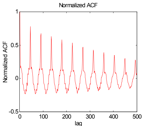
Fig. 3 The normalized autocorrelation of the real data s_1
