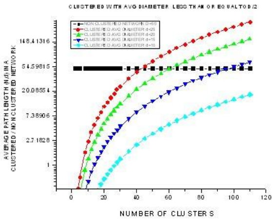
Fig. 6. Path Length (Upper bound) with respect to D
