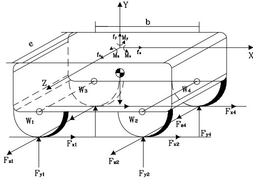
Fig. 2 Free body diagram of the vehicle
