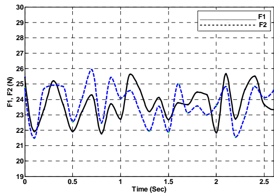
Fig. 8 Upward forces of tires number 1, 2
