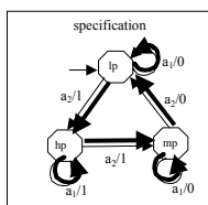
Fig. 5 Test generation based on TT method
