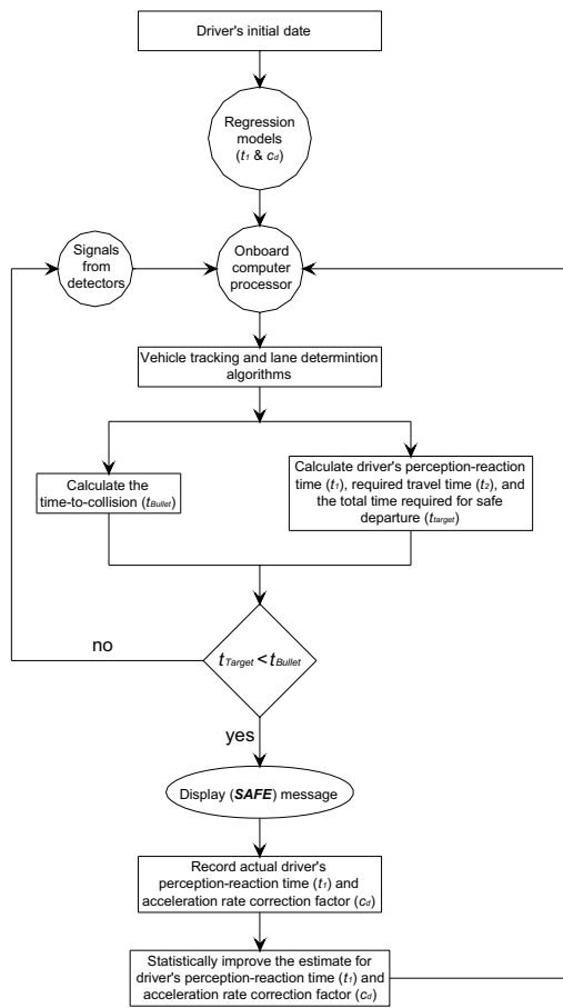
Fig. 2 Flow chart for the proposed algorithm
