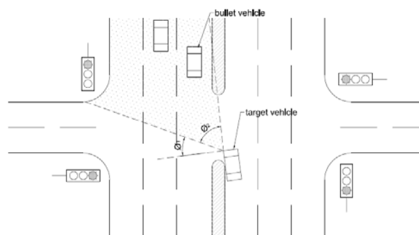
Fig. 1 System configuration
