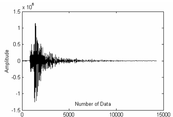
Fig. 3 East-West Component of Bala/Turkey earthquake
