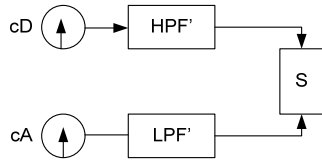
Fig. 2 DWT reconstruction
