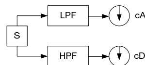
Fig. 1 DWT Decomposition
