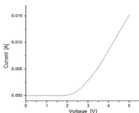
Fig. 3 I-V curve observed at room temperature
