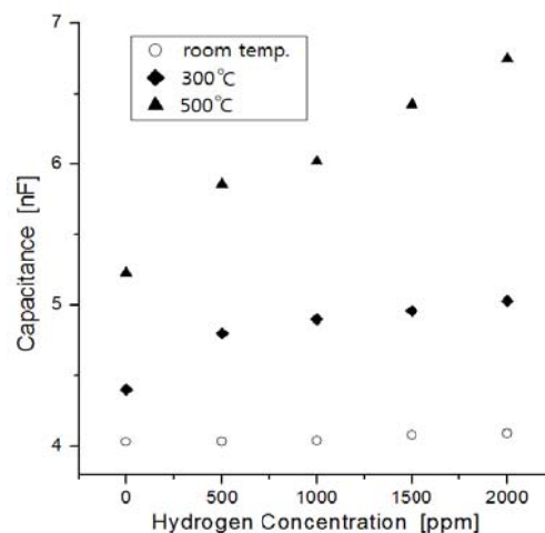
Fig. 4 Dependence of capacitance on hydrogen concentrations as a function of temperature
