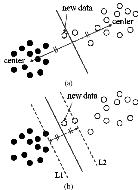
Fig. 2 Comparison of (a) general linear classification method with (b) SVM
