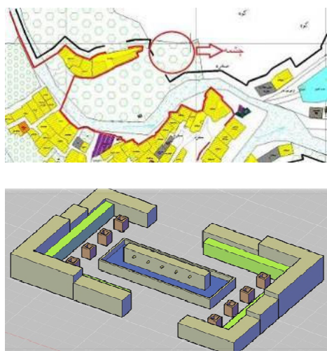
Fig 5 Main spring location and proposed plan to improve the spring, Ushtobin Village
