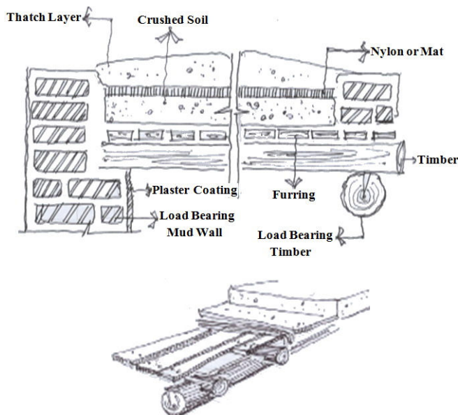
Fig 16 Roof covering details in Ushtobin Village Houses
