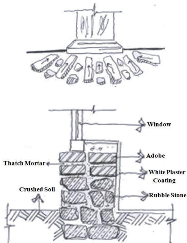
Fig.17: Wall details in Ushtobin Village Houses
