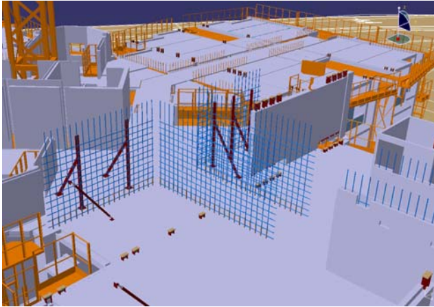
Fig. 6 Simulation of reinforcement fixing process
