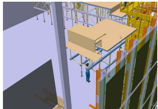
Fig. 4 Human movement simulation in detailed process analysis
