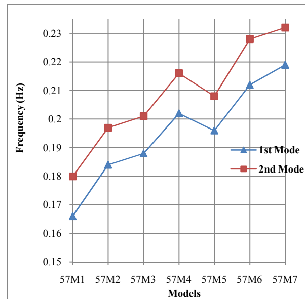
Fig. 11 Frequency comparison for 57-storey
