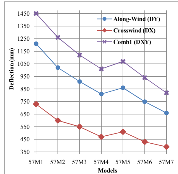
Fig. 10 Deflection comparison for 57-storey
