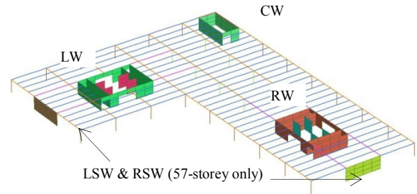
Fig. 3 Wall Designation
