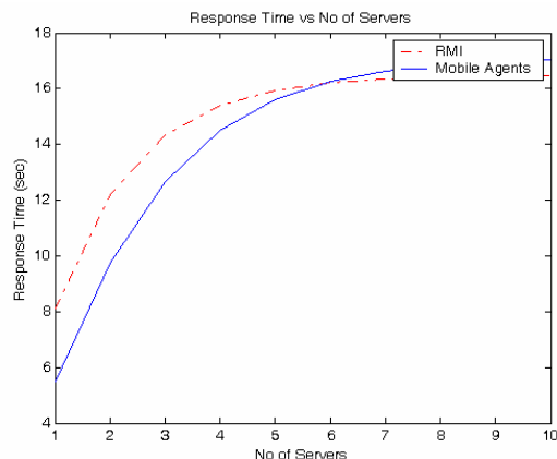
Fig. 6 Response time versus No of servers
