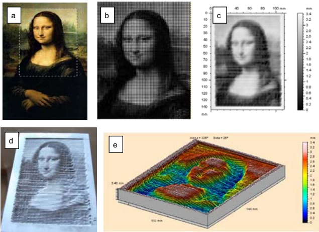
Fig. 5 Images showing important phases of spatial object (Mona Lisa) sculpturing basing on its photocopy: a- picture, b – virtual 2D matrix, c- image scanned from the relief, d- photo of 3D bas-relief cut in AlMg1SiMn plate. E-perspective scanned view showing depth analysis
