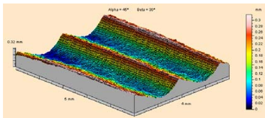
Fig. 6 Shape regularity and edge height of respective jet paths after AWJ treating of AlMg1SiMn for p=40 MPa, garnet #120, m_a=0.56 g/s
