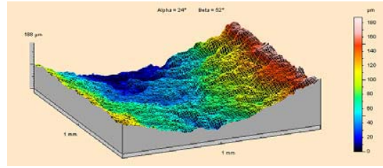
Fig. 7 Quality of the bottom of eroded region for AWJ treating of AlMg1SiMn (p=50 MPa, garnet #120, m_a=0.90 g/s)
