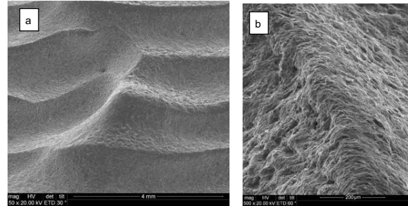
Fig. 8 Typical configuration of macro- (a) and micro- (b) surface eroded in aluminum alloy (AlMg1SiMn, p=40MPa, garnet #120, m_a=0.56 g/s)
