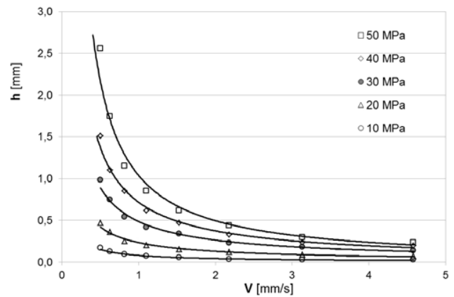
Fig. 3 AlMg1SiMn erosion realized with AWJ technology (garnet #120, m_a=0.90 g/s)
