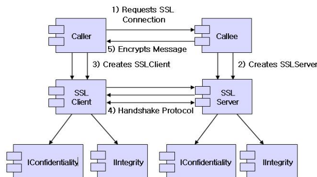
Fig. 3 Transmission of the RMI-based SSL Message
