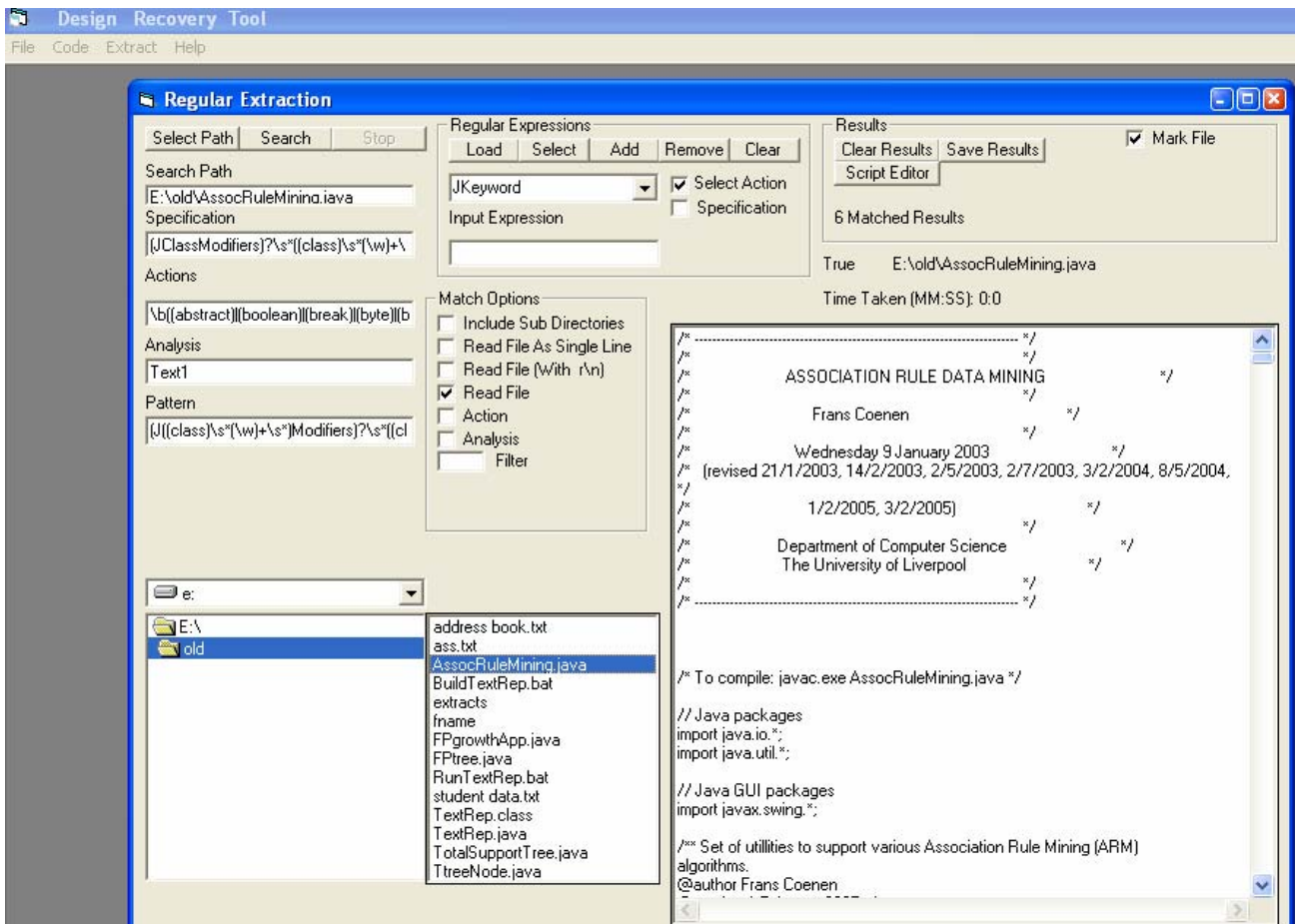
Fig. 2 Screen Snapshot of DRT
