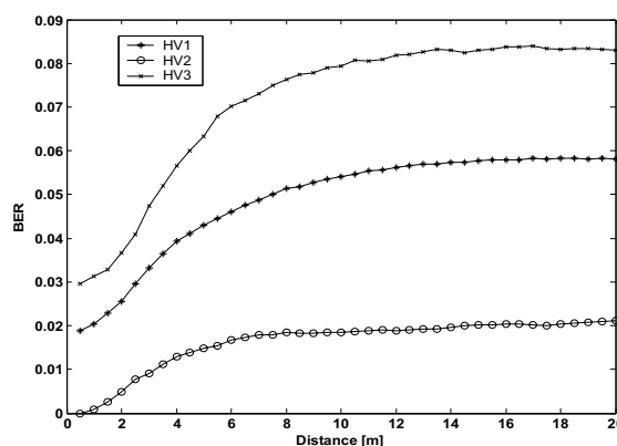
Fig. 5. BER versus distance between the master and the slave
