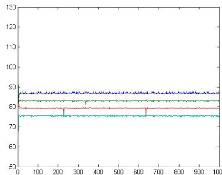
Fig. 4. Exponential model. First outer loop.
