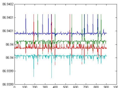
Fig. 3. Polynomial model. Third outer loop.
