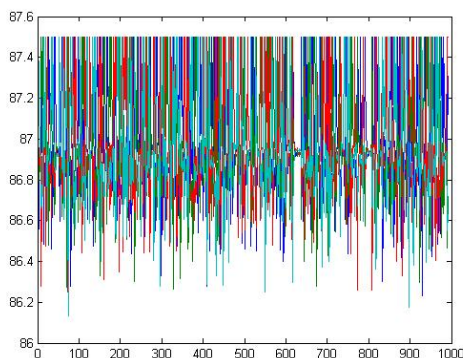
Fig. 2. Polynomial model. First outer loop.
