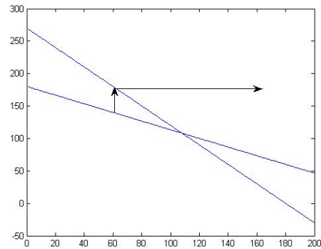
Fig. 1. Best replies in Arifovic’s model
