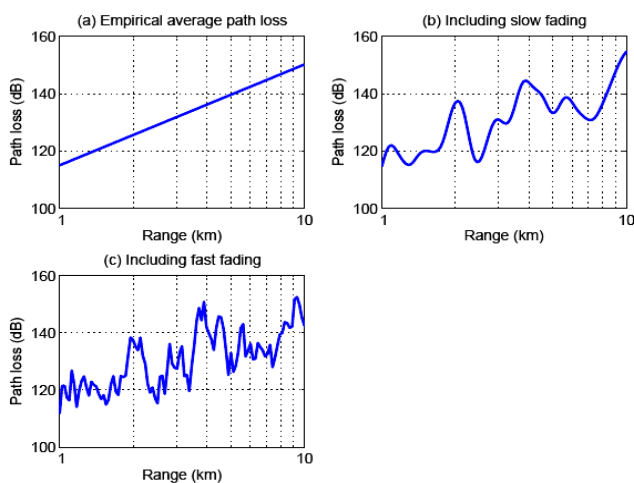
Fig. 3: Depiction of classic path loss behaviours; (a) Expected path loss w.r.t. an empirical model, (b) path loss behaviour with slow fading effects included, (c) path loss behaviour with the effects of fast fading additionally included (Source: [6])
