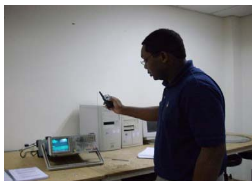
Fig. 9: Emmanuel Ojakominor carries out preliminary checks on transmit and receive devices before commencing actual measurements. Notice the transmit device (walkie-talkie, model T-388, with output power approximately 0.5W) and the receive equipment (Tektronix 2711 spectrum analyser along with a simple telescopic antenna)
