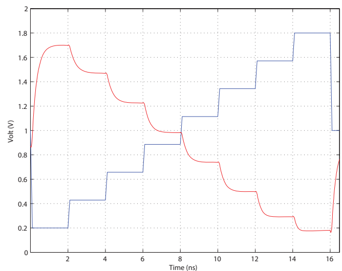
Fig. 2. The simulation result for the pseudo floating-gate inverter in the context of MVL. A single input PFG in continuous mode with input ranging from 0.2V to 1.8V with a frequency of 500MHz. The steps are a little smaller compared with the input, but are justifiable within the noise margin.
