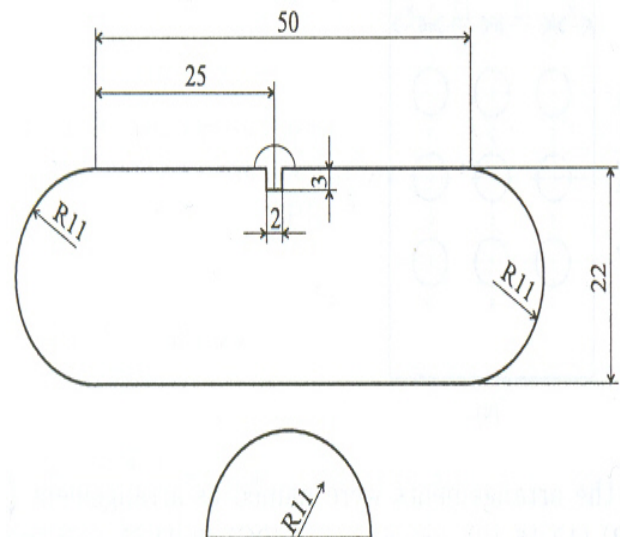
Fig. 1 Top view (above) and cross section (bottom) of the electrodes used (all dimensions in mm)
