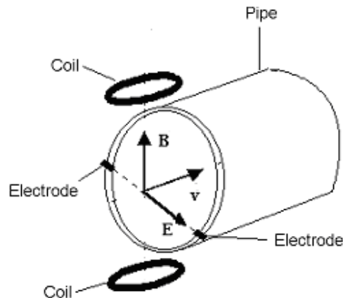
Figure 1: Cross-section of an EMFM.
