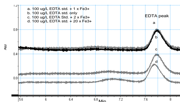
Fig. 5 Overlay of chromatograms by adding different levels of iron to a 100 μg L -1 EDTA standard solution. Conditions: Column, Hypersil C 18 RP column (Phenomenex) of length 200 mm, diameter 4.6 mm and particle size 5 μm; Mobile phase, 2% MeOH, 15 mM TBABr in pH 3.3 sodium formate/formic acid buffer solution; sample loop, 50 μL; Flow rate, 0.9 mL min -1 ; Wavelength, 265 nm
