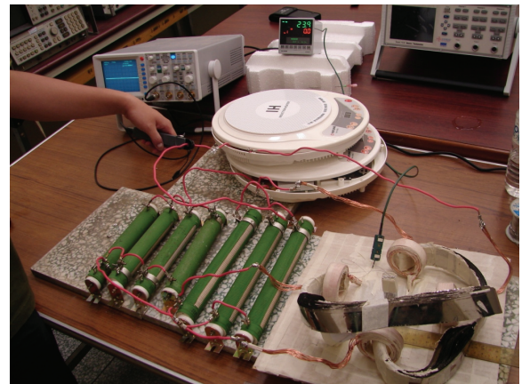
Fig. 5 System with two pairs of Helmholtz coil
