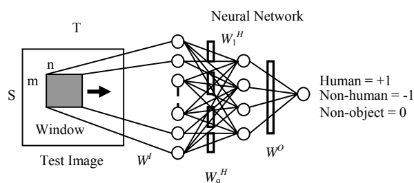
Fig. 6 The MLP neural network structure used
