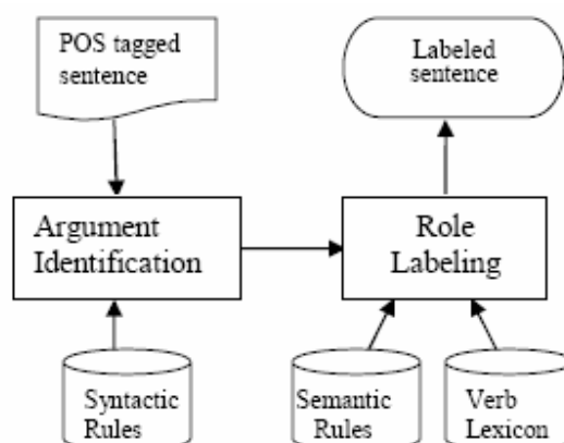
Fig. 1 The Thematic Role extraction system architecture
