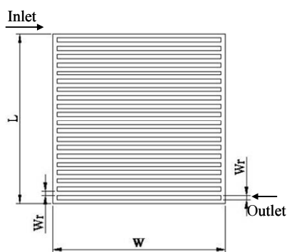
Fig. 1 PEMFC with parallel channel physical model
