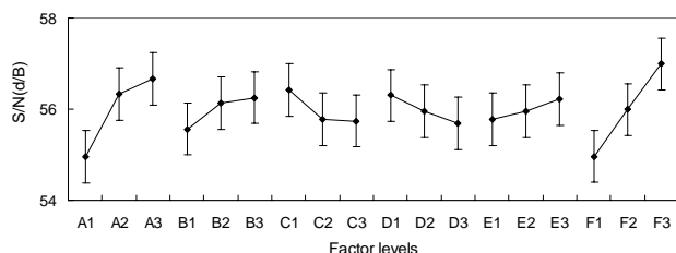
Fig. 5 S/N response graph for power density
