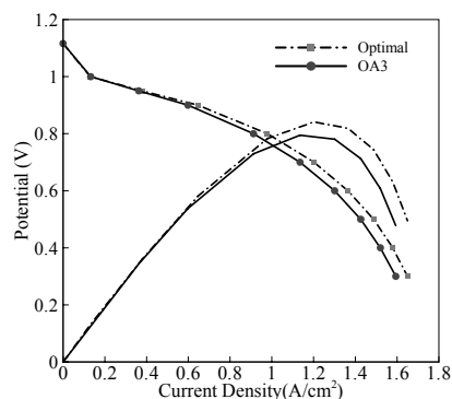
Fig. 6 Comparisons of I-V curves between original (OA3) and optimum results
