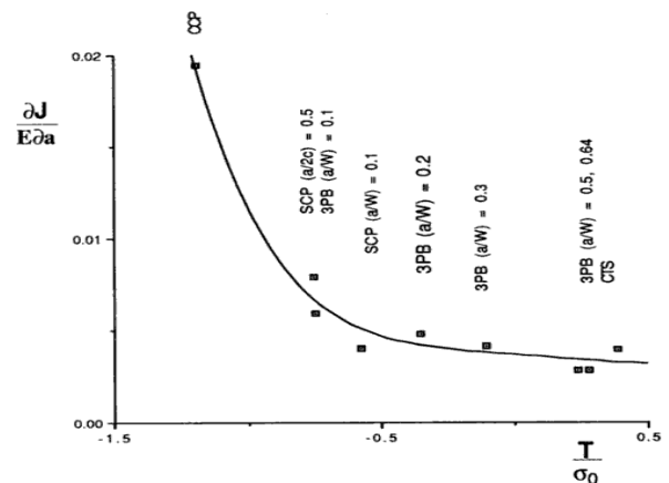
Fig. 4 The slope of the J- \Delta a resistance curve as a function of T [11]
