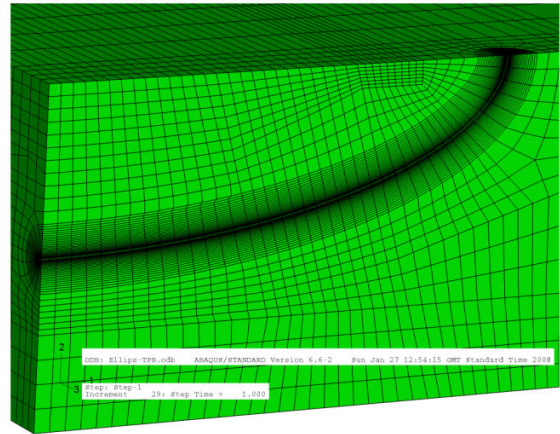
Fig. 3 The mesh for a semi-elliptical surface crack
