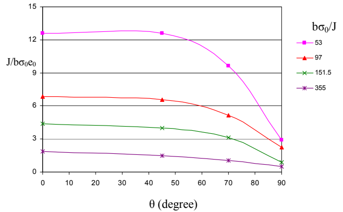
Fig. 12 J-integral along the crack front for a deep semi-elliptical surface crack in tension, a/c=0.33 , a/w=0.5
