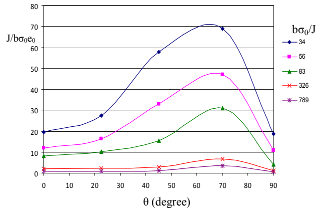
Fig. 8 Non-dimensional J-integral along the crack front in a semi-elliptical surface crack ( a/w=0.5 , a/c=0.33 ) in bending
