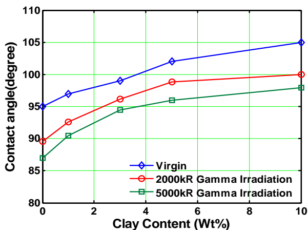
Fig. 3 Variation in contact angle of epoxy nanocomposites
