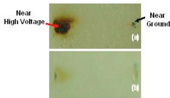
Fig. 9 Typical erosion structure observed with different current limiting resistors (a) 10 MΩ (b) 20MΩ
