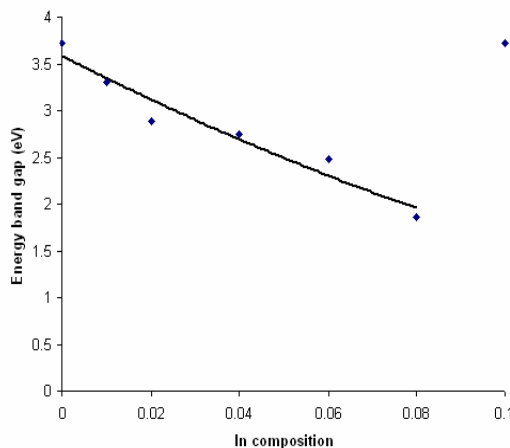
Fig. 3 The energy band gap versus In composition plot of \text{In}_x\text{Al}_y\text{Ga}_{1-x-y}\text{N}
