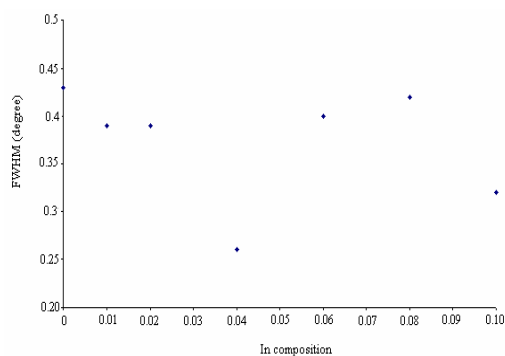
Fig. 2 Full width at half maximum (FWHM) intensity of the (0002) quaternary \text{In}_x\text{Al}_y\text{Ga}_{1-x-y}\text{N} alloys as a function of the In mole fraction using XRD rocking curve
