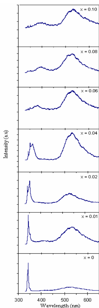
Fig. 4 Room temperature of PL spectra for \text{In}_x\text{Al}_y\text{Ga}_{1-x-y}\text{N} with constant Al ( y = 0.06 ) and different In composition, x (varied from 0 to 0.1)
