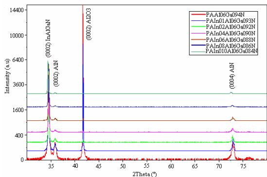
Fig. 1 XRD Phase analysis of \text{In}_x\text{Al}_y\text{Ga}_{1-x-y}\text{N} quaternary alloys
