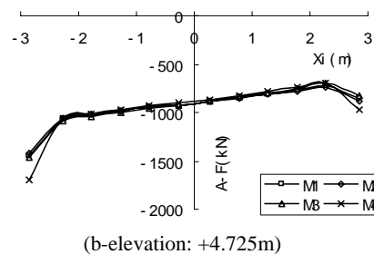
Fig. 4 Axial force distribution of columns
