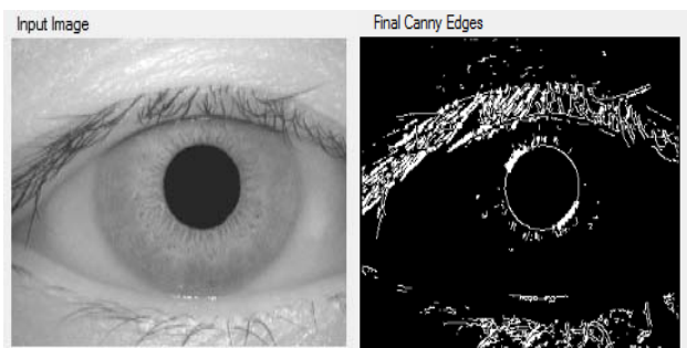
Fig. 8 Final Edges – Hysteresis thresholding by TH=40, TL=20
