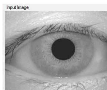
Fig. 4 Original Image
