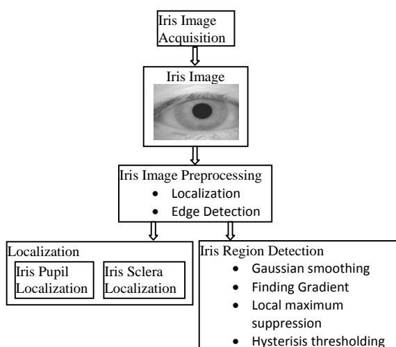
Fig. 1 Flow diagram of the proposed system
