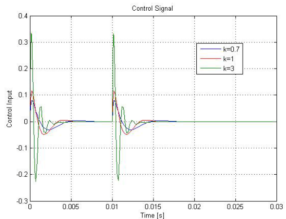
Fig. 8. Control Signal of Controller
