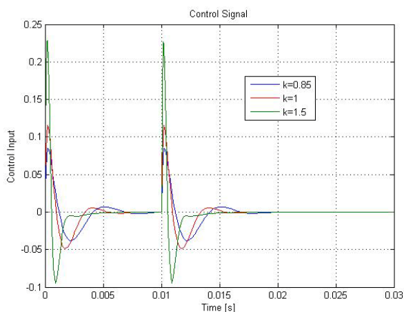
Fig. 10. Control Signal of Controller
