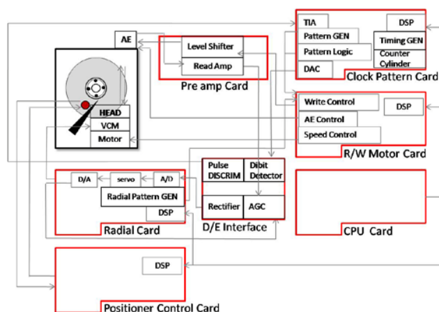
Fig. 1. Block Diagram of One Cell Tester
