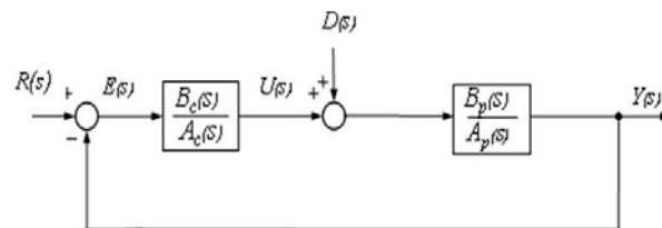
Fig. 4 A block diagram of CDM control system.
