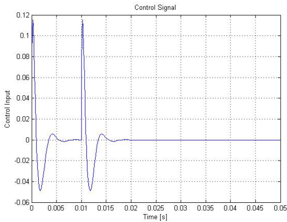
Fig. 6. Control Signal of Controller
