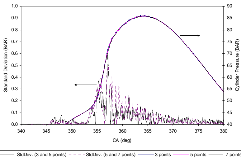
Fig. 3 Smoothing technique effect of 3, 5 and 7 points moving average on cylinder pressure curve with their standard deviation at 1200 RPM and 150 N.m using AD
