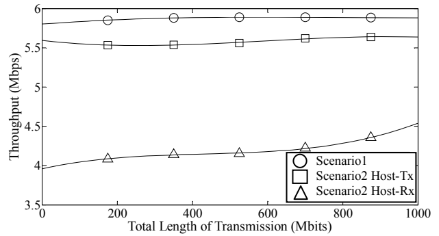
Fig. 4 Throughput, Scenario 1 Vs Scenario 2
