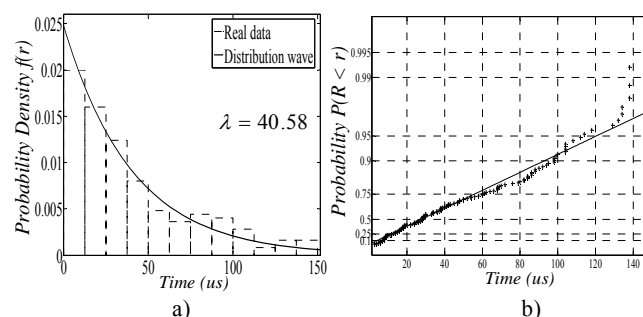
Fig. 14 Exponential function distribution for inter-arrival times a) PDF b) Exponential probability
