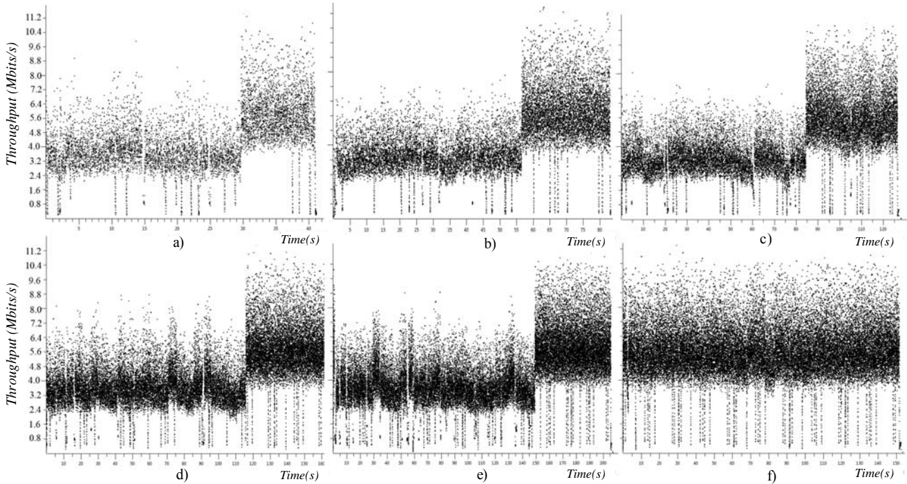
Fig. 5 Scenario 2 at Rx side, with files of a) 20MB, b) 40MB, c) 60MB, d) 80MB and e) 100MB. f) At the Tx-side with 100MB
