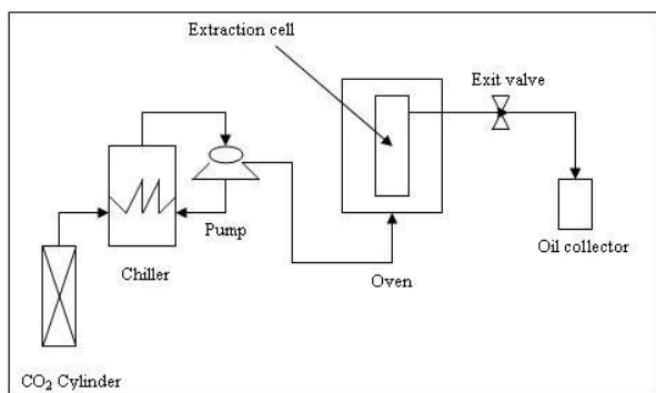
Fig. 1 Supercritical Fluid Extraction Apparatus
