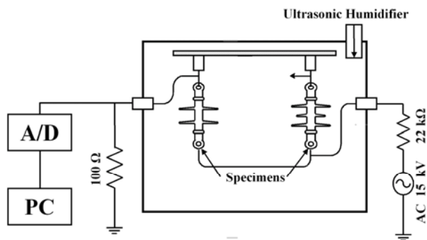
Fig. 2 Test Arrangement
