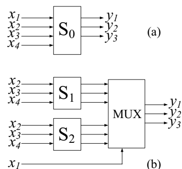
Fig. 14. Shannon decomposition.
