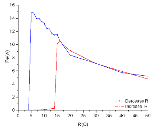
Fig. 9 Fig. 10 Hysteresis relationship between output power ( P_e ) and external resistance ( R ) for wind speed 7 m/s
