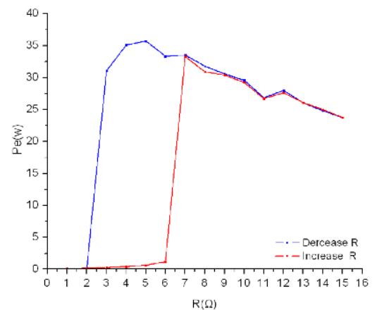
Fig. 10 Hysteresis relationship between output power ( P_e ) and external resistance ( R ) for wind speed 9 m/s
