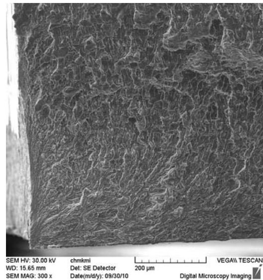
Fig. 1 Initiation Of Fatigue Crack At Corner Edge Of Material Treated By Nitrooxidation
