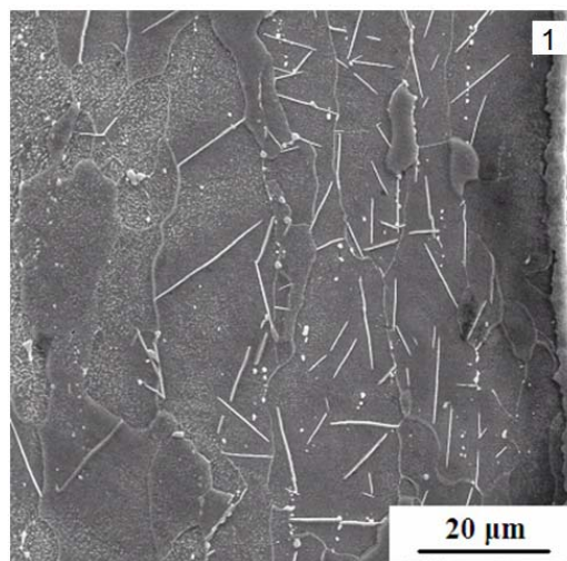
Fig. 2 Coarse needles of Fe 4 N nitrides
