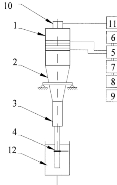
Fig. 6 Scheme of testing equipment KAPU
